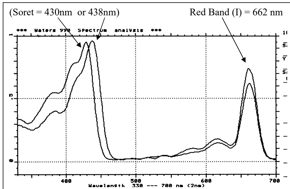
Figure R8: The absorption (PDA) spectra of 'regular'(monovinyl) chlorophyll-a (S= 430nm) and of divinyl chlorophyll-a (S= 438nm).
